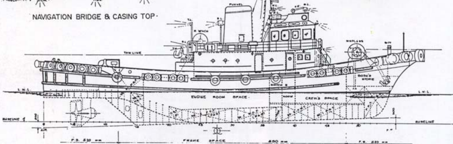
OUTBOARD PROFILE
