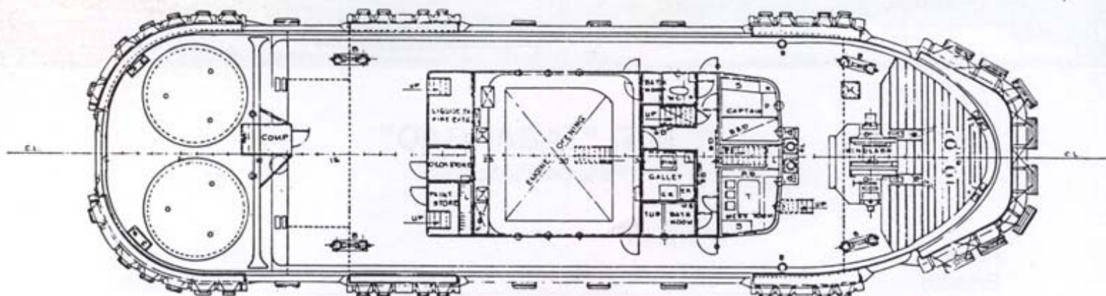
UPPER DECK PLAN
