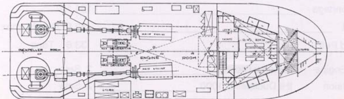
UNDER DECK
