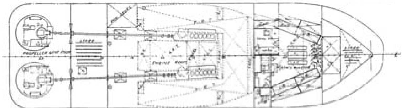
HOLD PLAN
