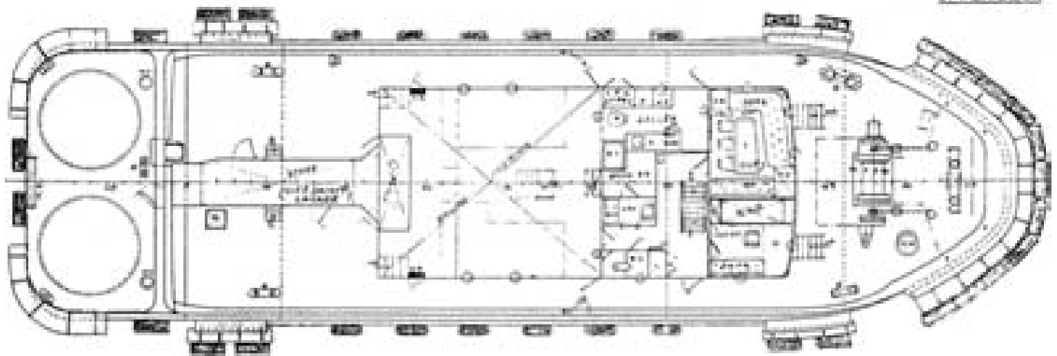
UPPER DECK
