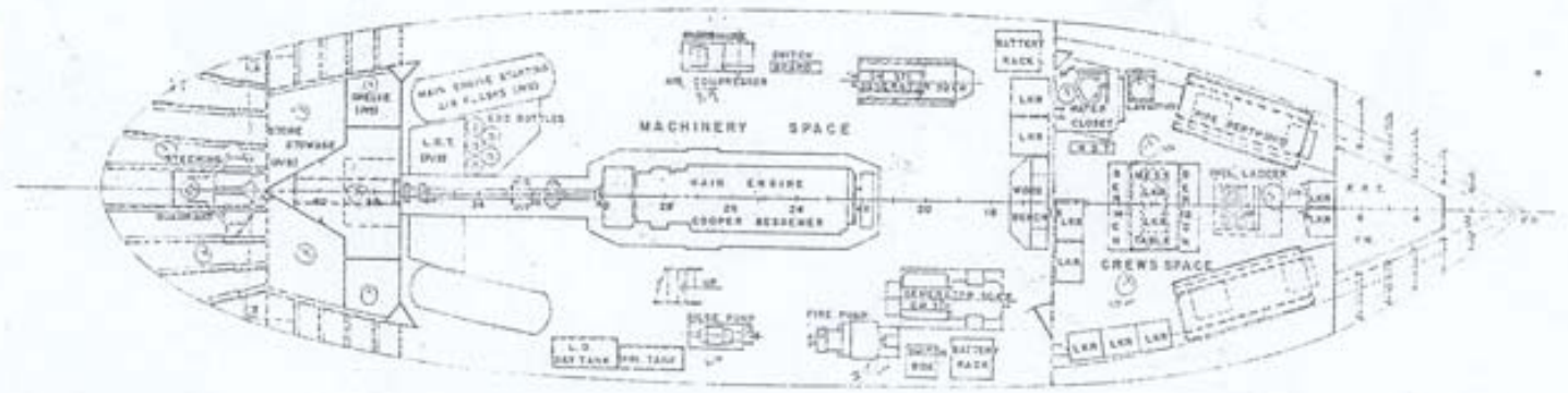
HOLD ARRANGEMENT
