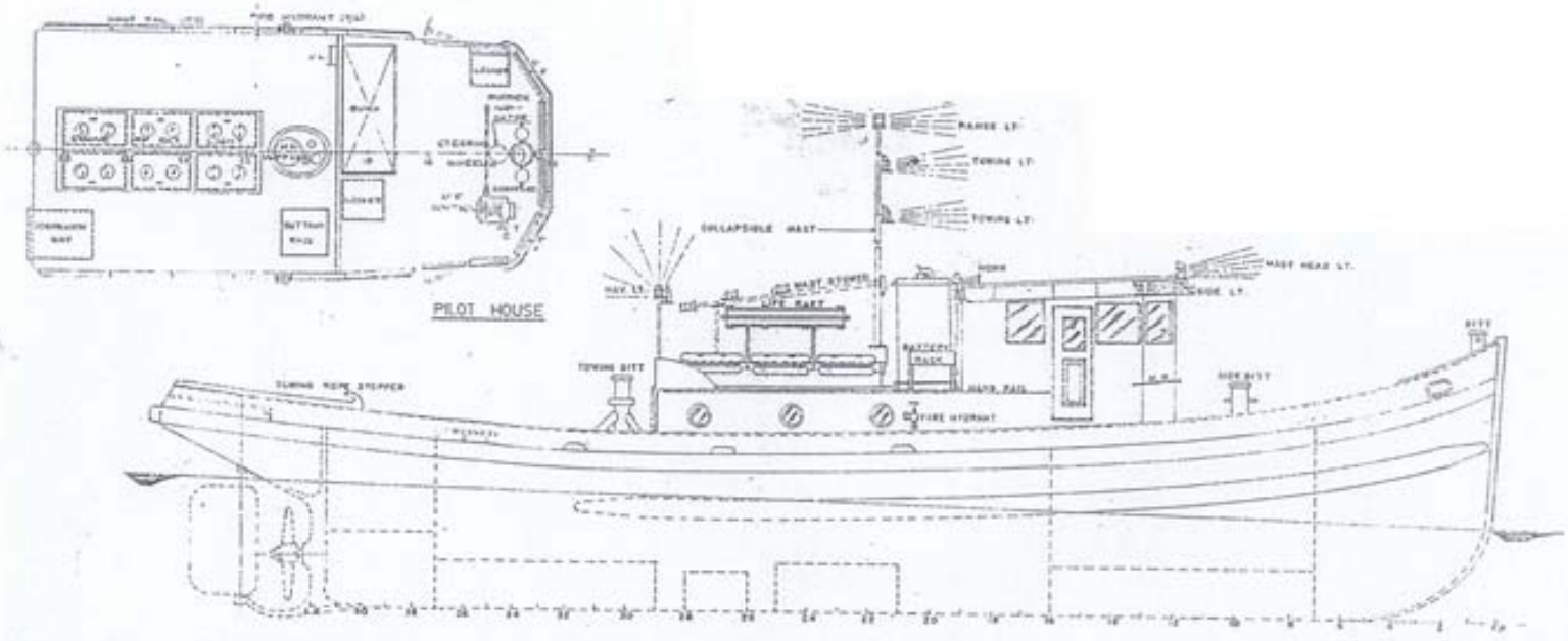
OUTBOARD PROFILE
