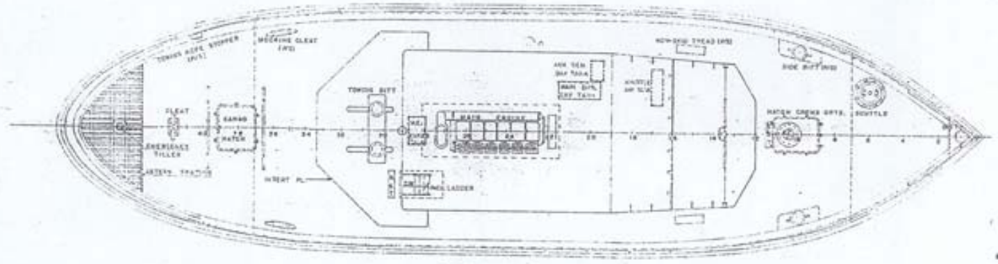
DECK ARRANGEMENT
